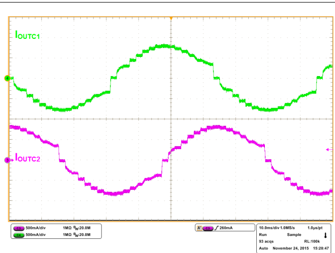
Figure 14. 1/8 Step Microstepping with Slow Decay
