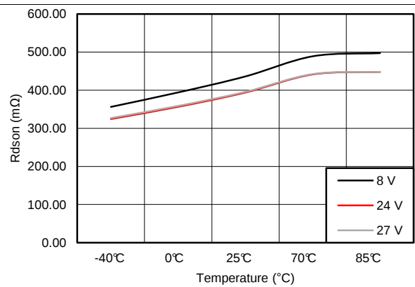
Figure 9. HS R_{DS(on)} A_{OUT1} over Temperature
