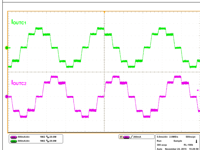
Figure 15. 1/2 Step Microstepping with Mixed Decay
