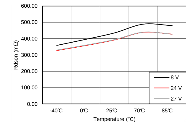
Figure 8. HS R_{DS(on)} A_{OUT2} over Temperature
