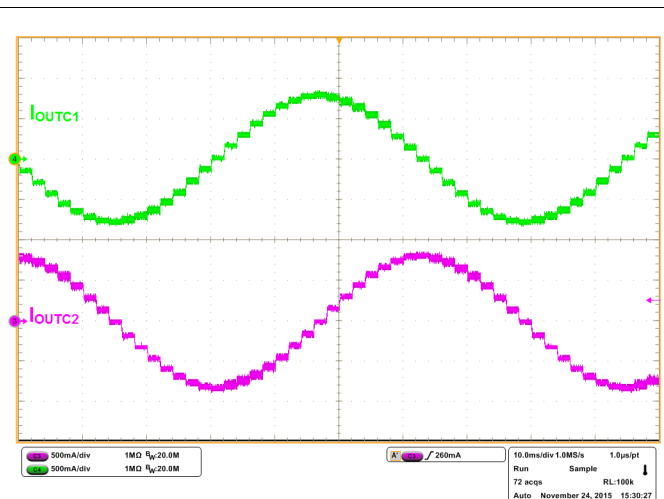
Figure 16. 1/8 Step Microstepping with Mixed Decay
