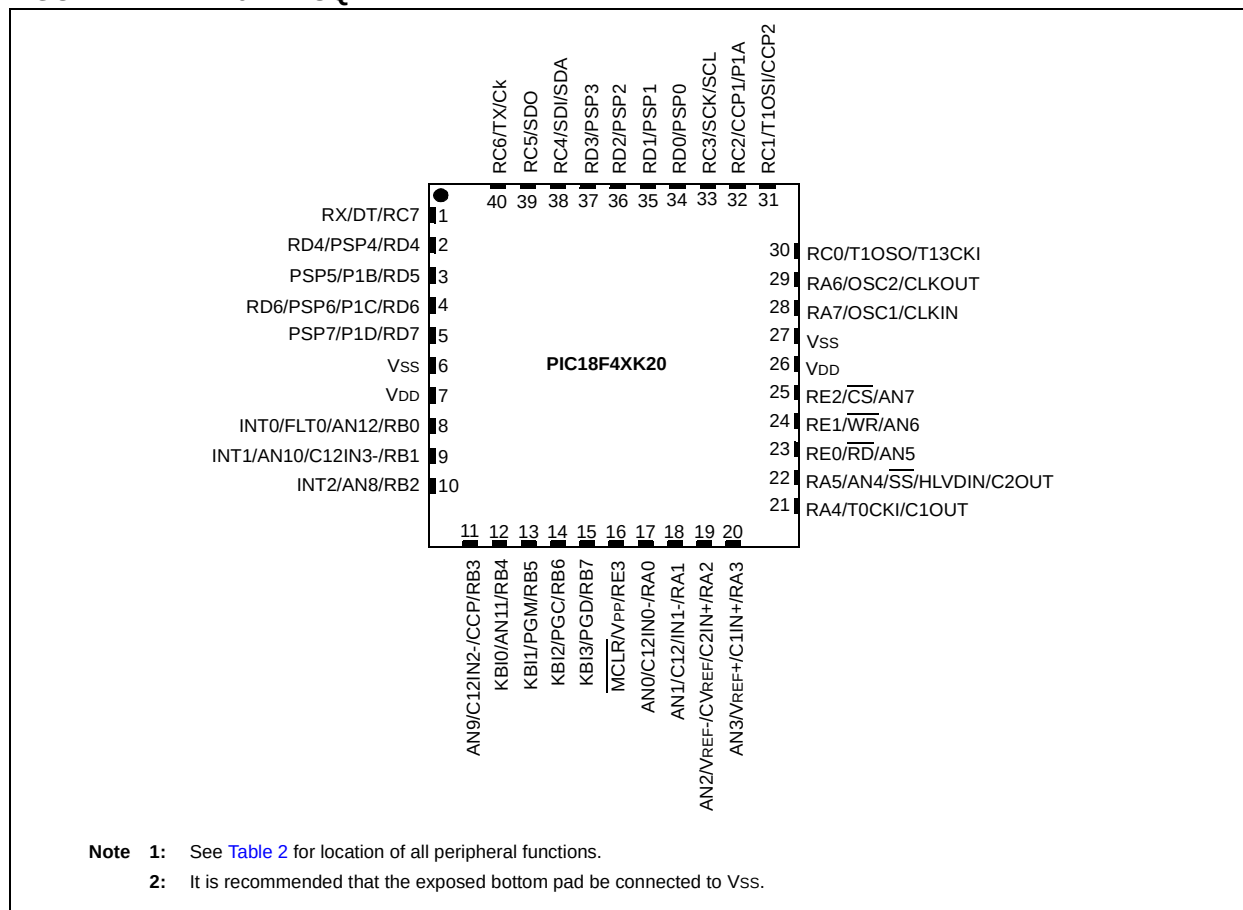
FIGURE 4: 40-PIN UQFN
