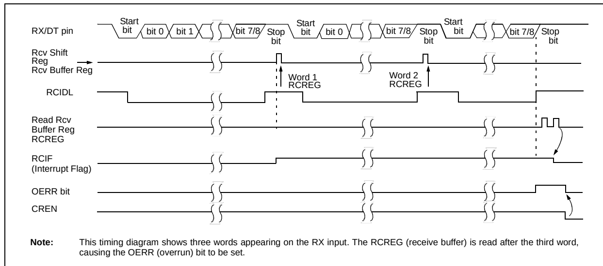
FIGURE 18-5: ASYNCHRONOUS RECEPTION
