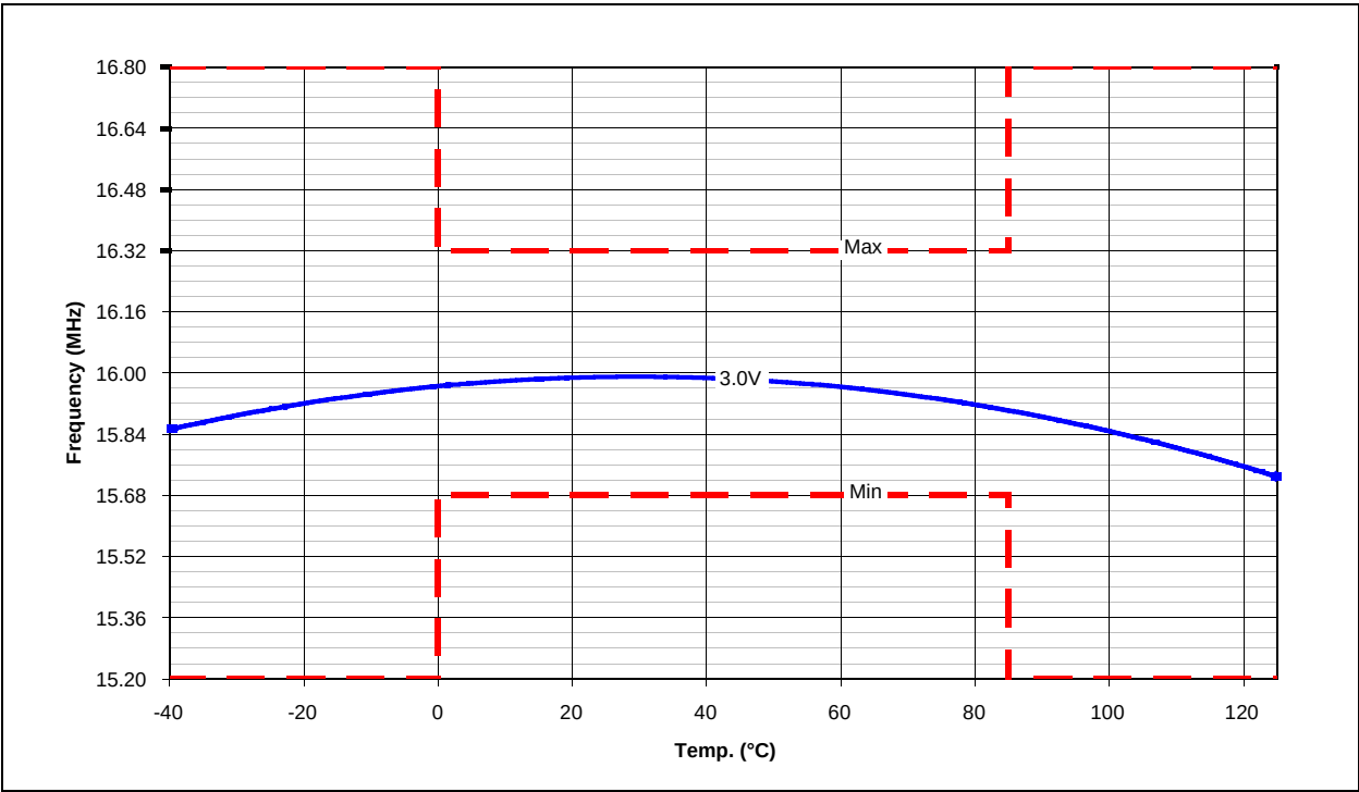
FIGURE 27-43: PIC18F4XK20/PIC18F2XK20 TYPICAL HF-INTOSC FREQUENCY
