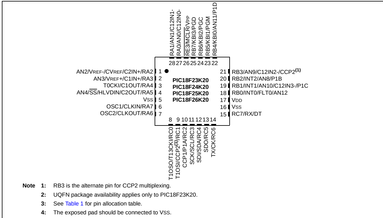
FIGURE 2: 28-PIN QFN/UQFN
