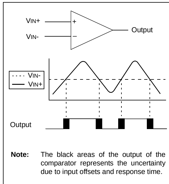
FIGURE 20-1: SINGLE COMPARATOR
