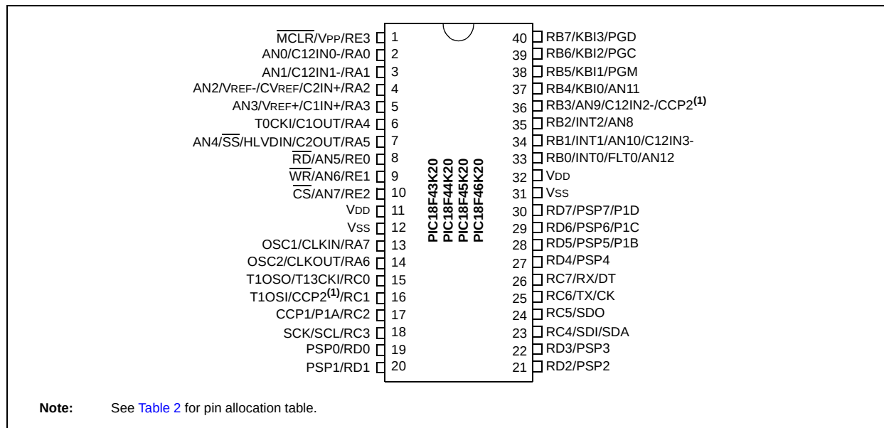
FIGURE 3: 40-PIN PDIP
