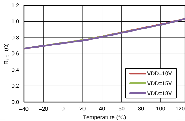
Figure 28. HO Output Pull-Down Resistance vs Temperature
